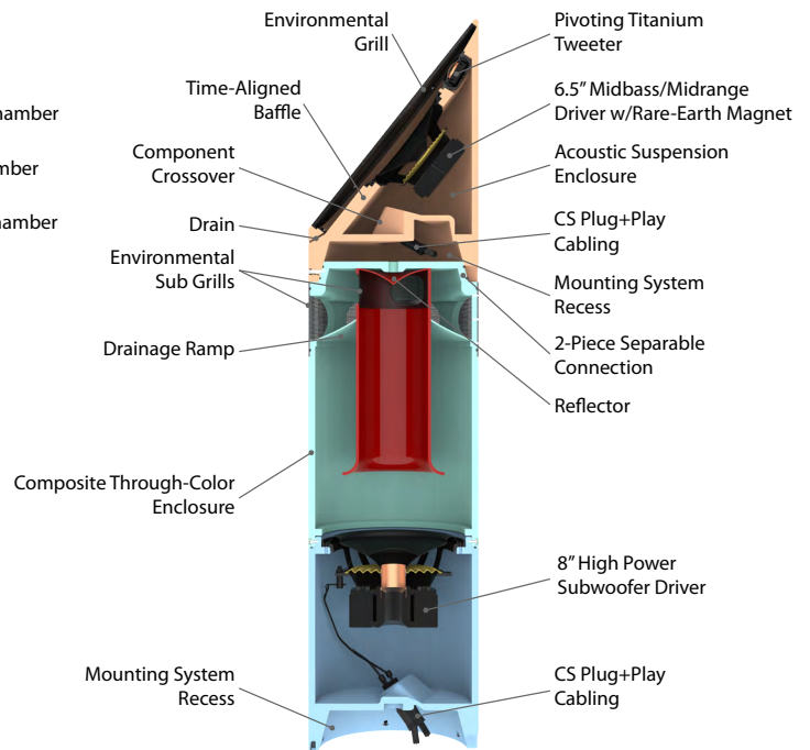
CROSS SECTION OF THE PATENTED 3-WAY ELLIPSE BOLLARD
